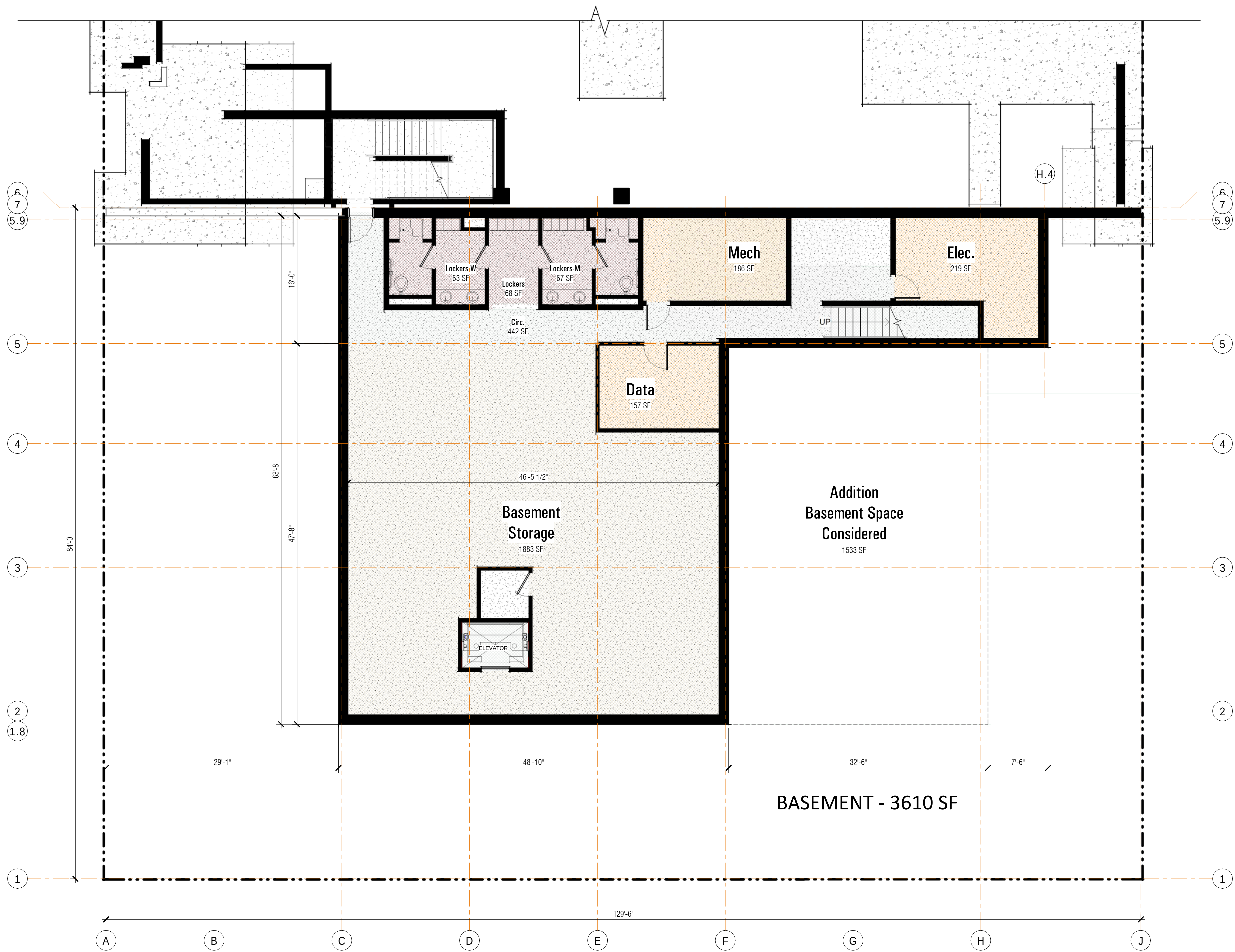
1 AA1-Level 00Basement 1/8" = 1'-0"
