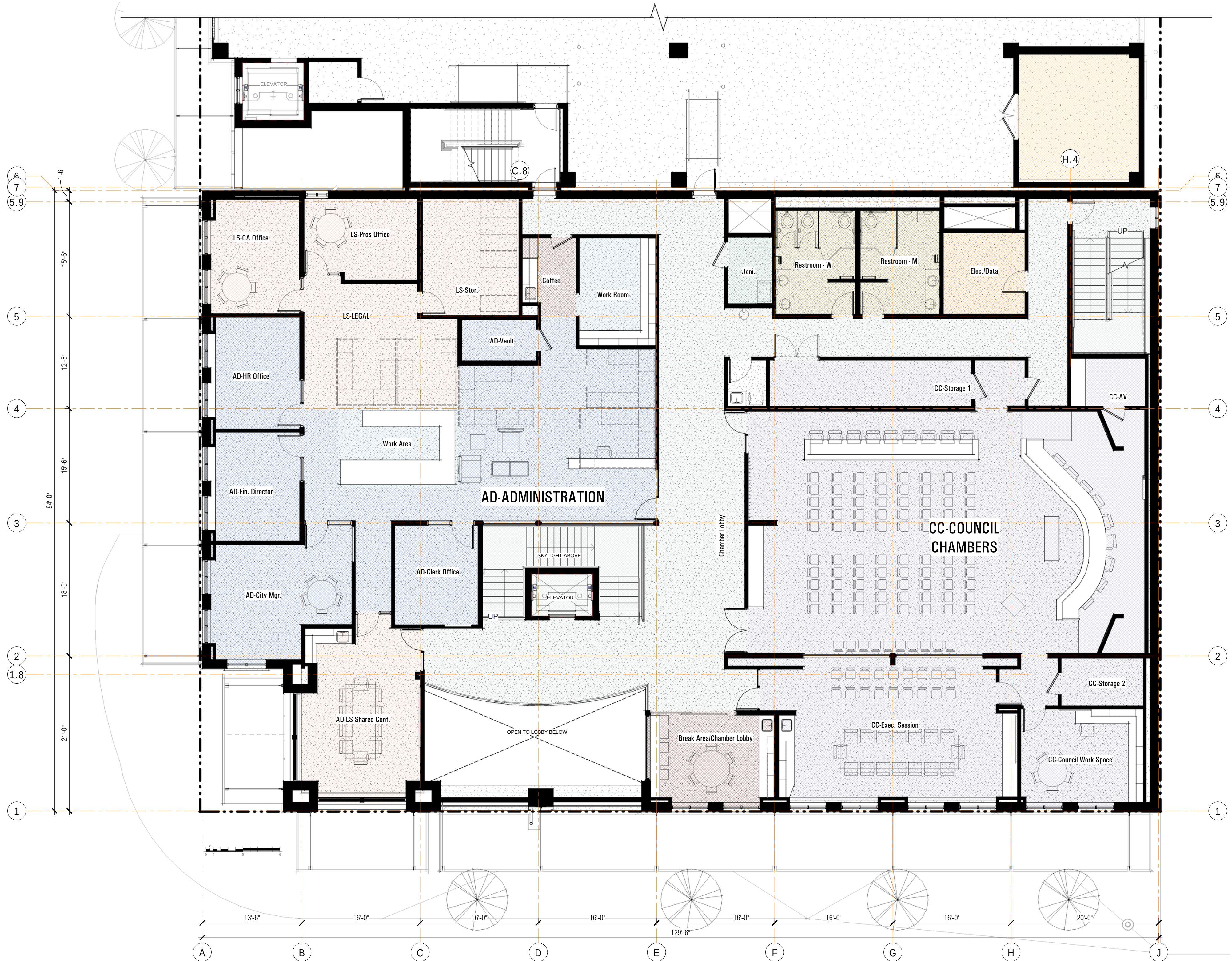
1 AA1-Level 02 1/8" = 1'-0"
