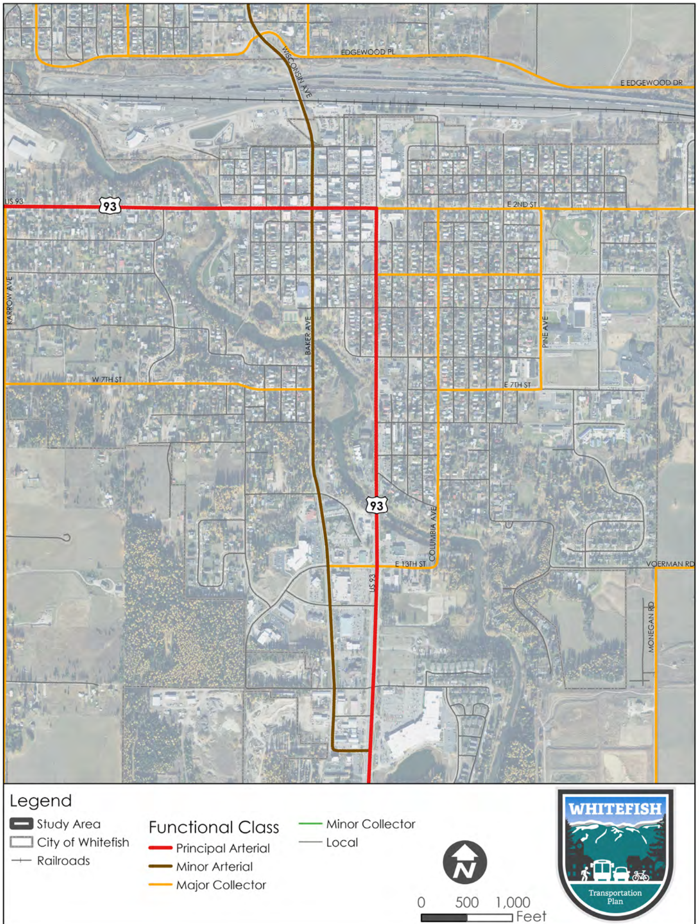
FIGURE 3.3: FUNCTIONALLY CLASSIFIED ROADWAYS IN THE STUDY AREA INSET
