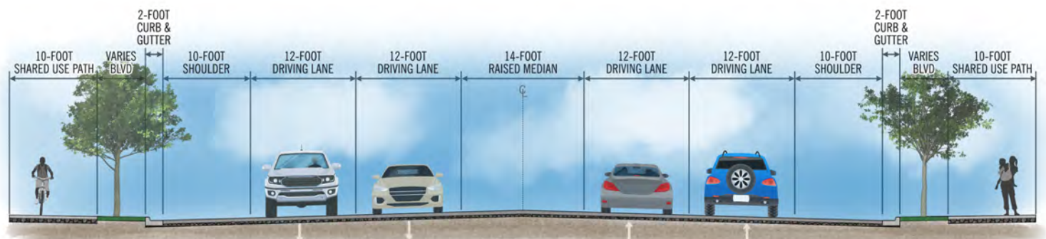
FIGURE 7.5: US-93 CORRIDOR TYPICAL SECTION
