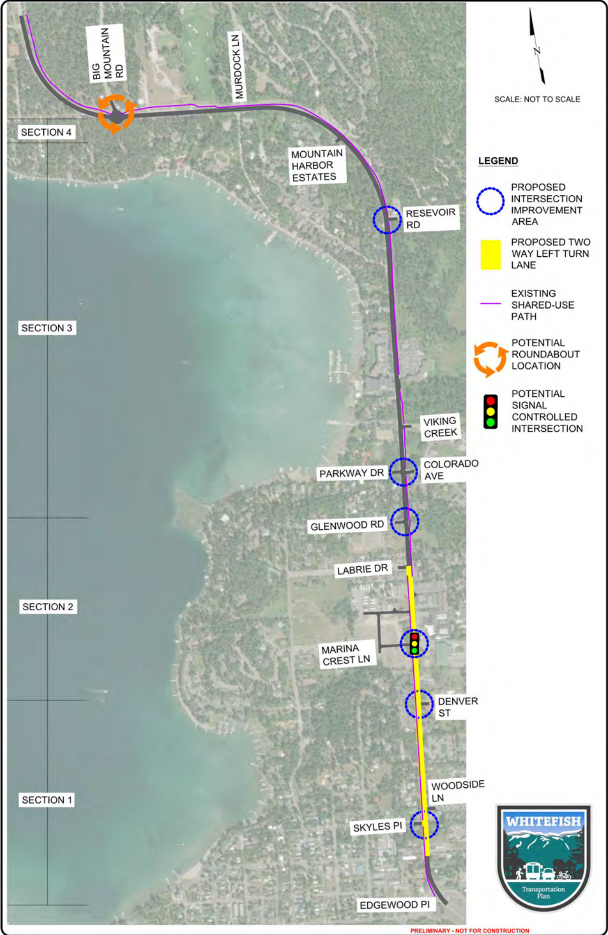
FIGURE 7.11: WISCONSIN AVENUE CORRIDOR PLAN AREA
